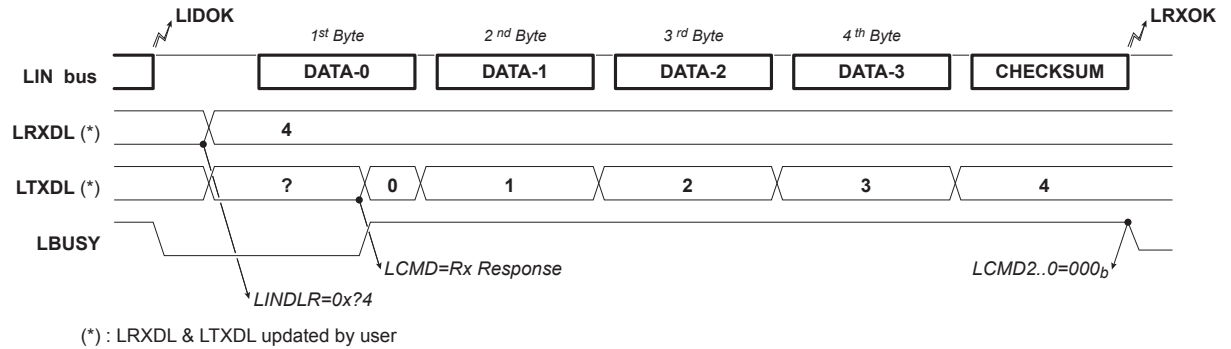
Figure 21-9. LIN2.1 - Rx Response - no error
