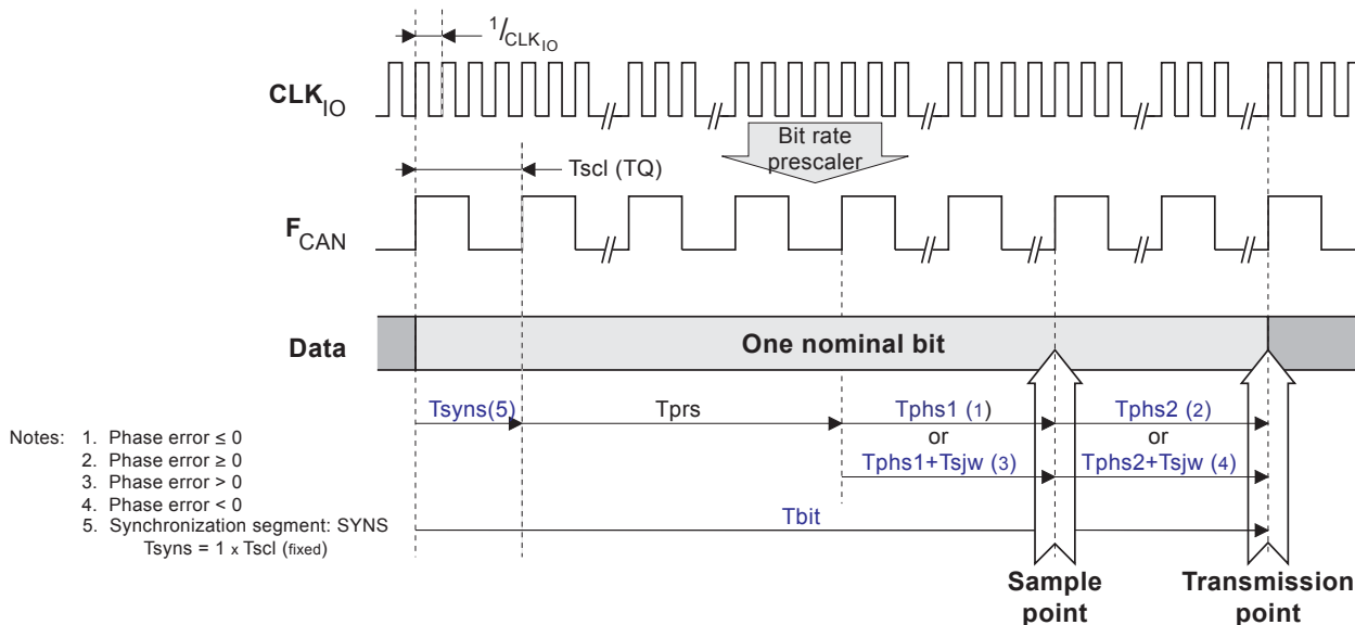
Figure 20-8. General Structure of a bit period
